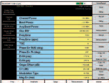
Option 41 provides a quick, table view of critical test parameters, including channel power, occupied bandwidth, phase error and EVM.
