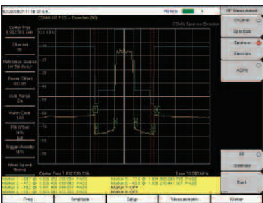
CDMA Spurious Emissions measurement display
