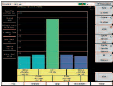
The ACLR screen shows the power levels for the main channel as well as two adjacent channels.
